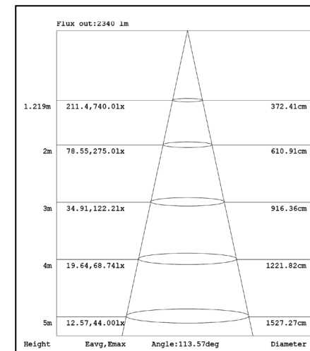
CURVE LUX/DISTANZA
