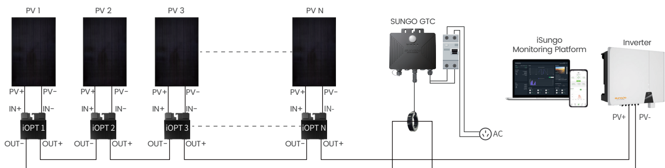
Connection Diagram
